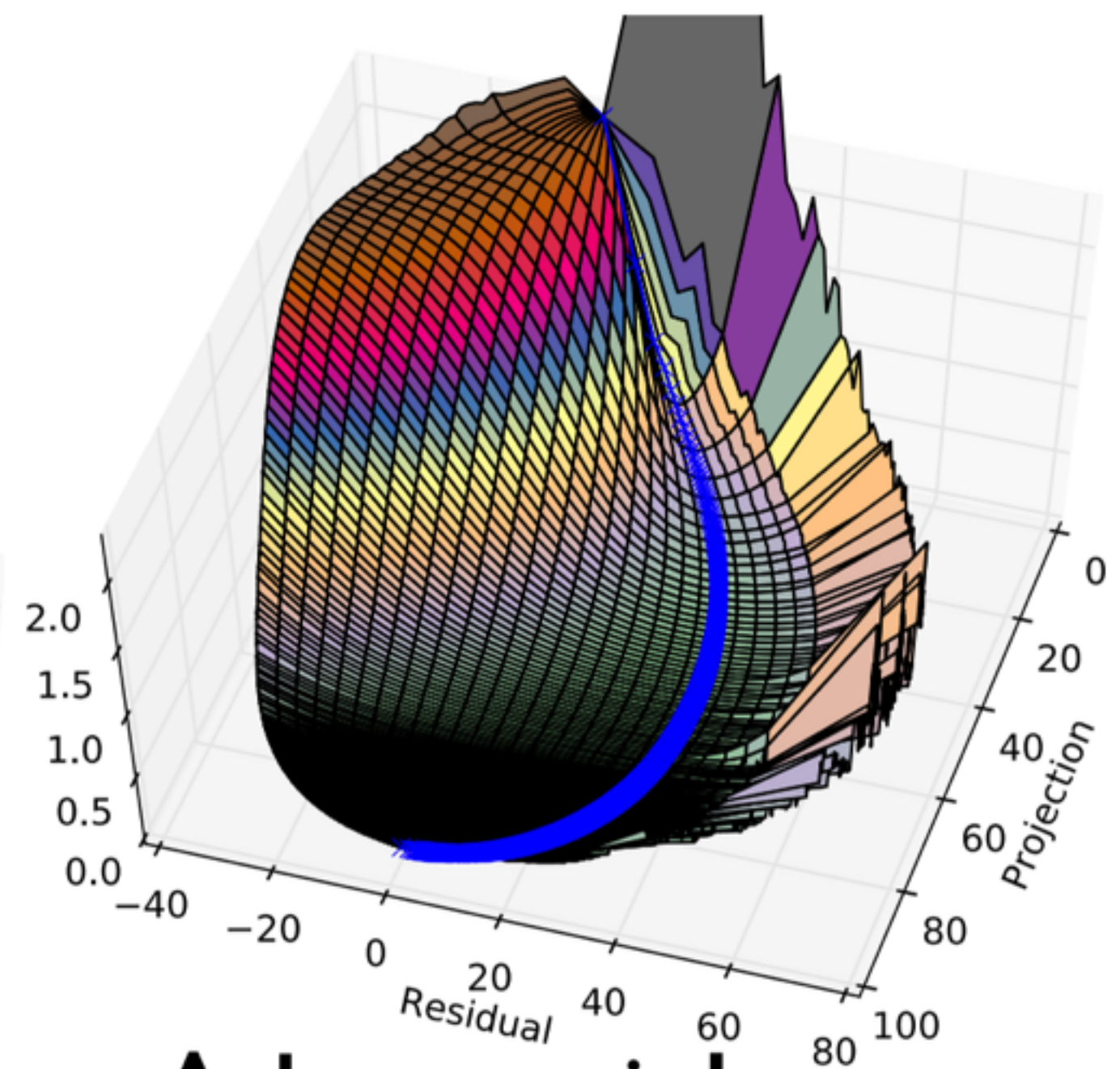
Adversarial ReLUs
