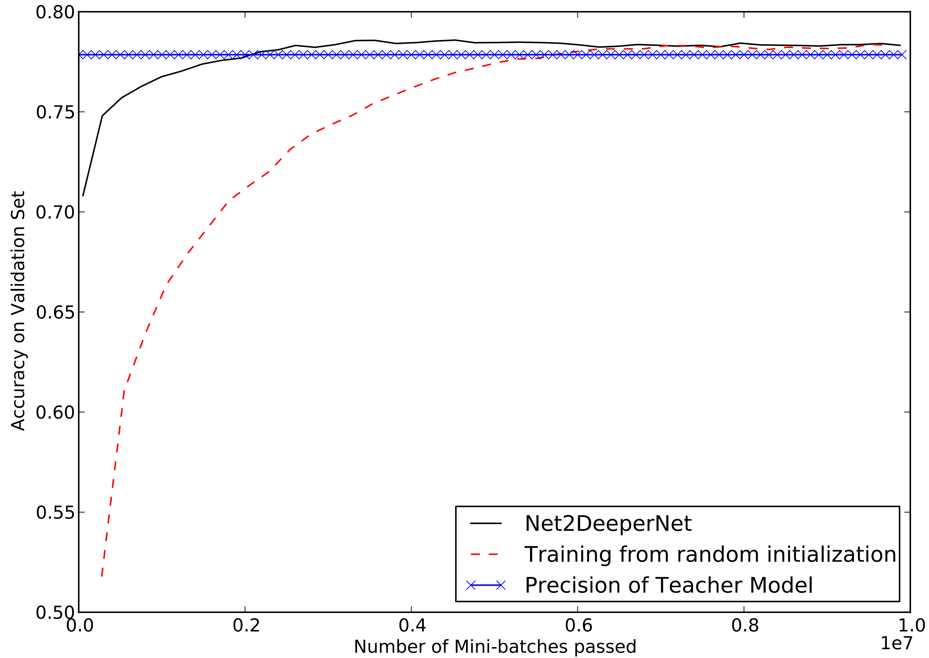
“Net2Net: Accelerating Learning via Knowledge Transfer.” Chen, Goodfellow, and Shlens, submitted to ICLR 2016
