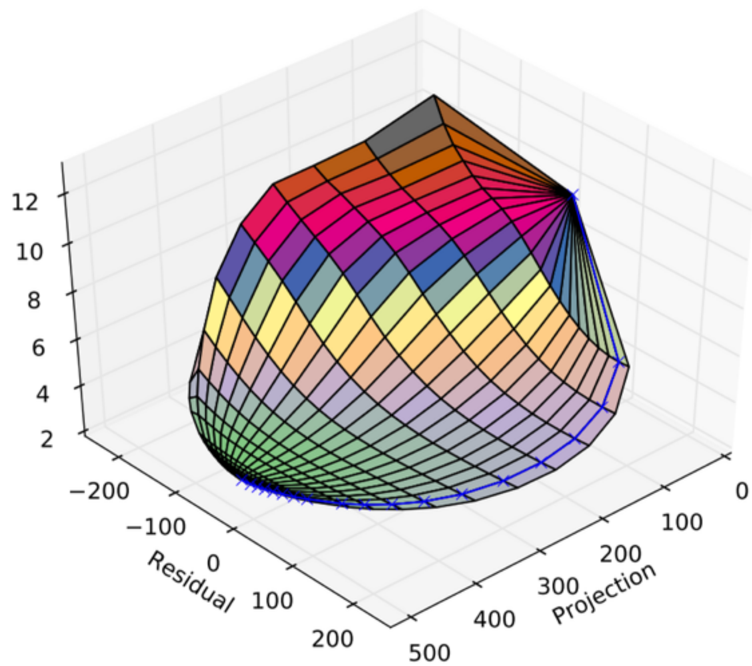
LSTM
